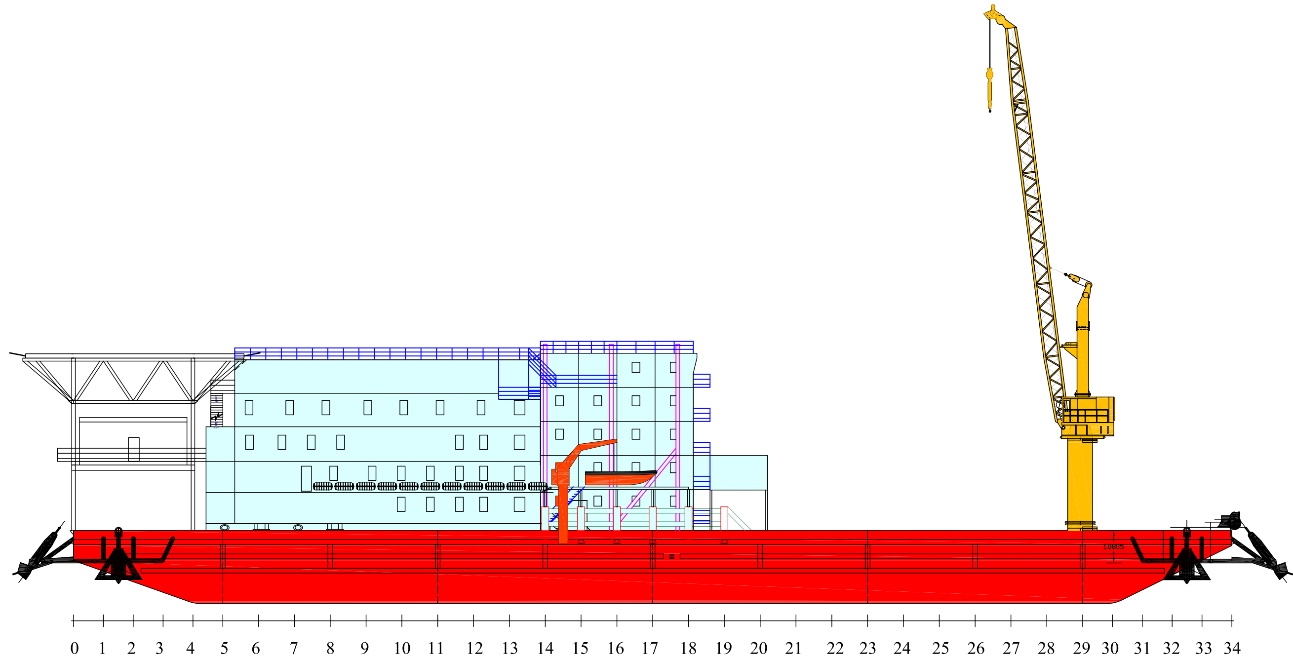
STBD. SIDE PROFILE
