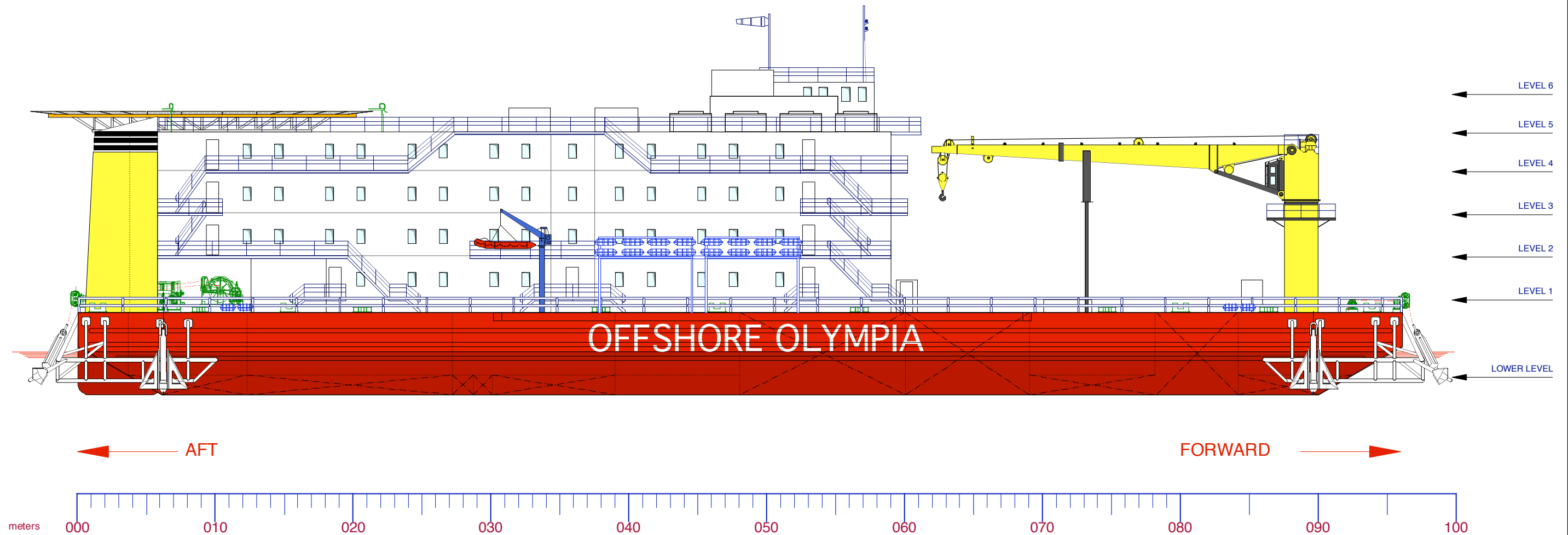
PROFILE (Starboard Side)
